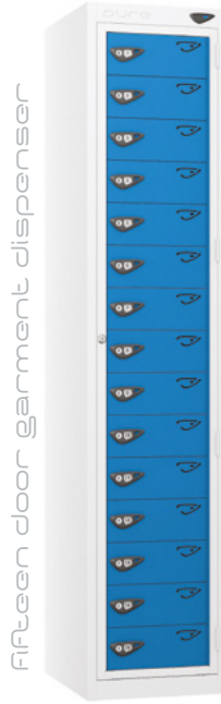
garment dispenser Width 380mm Depth 450mm Height 1800mm
